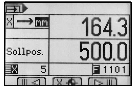
display structure 1-axis version
